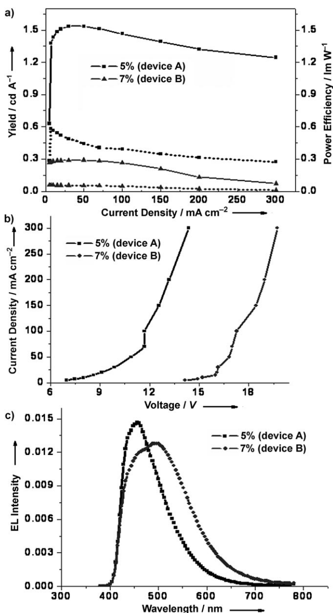
Figure 5. Electroluminescence (EL) performances of device A (5% complex 2 ) and device B (7% complex 2 ). a) Plots of luminescence yield (solid lines) and power efficiency (dotted lines), respectively, versus current density. b) Current density versus voltage curves. c) EL spectra of devices A and B.
